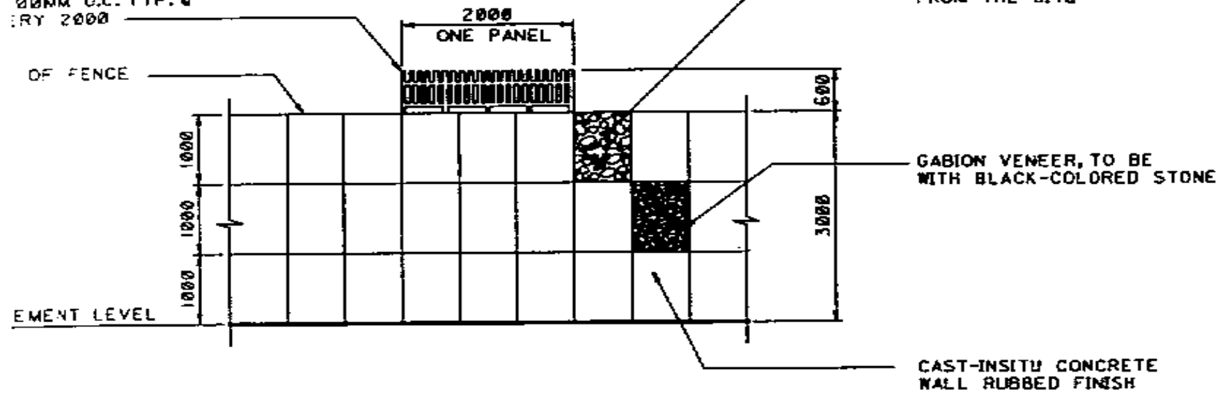
SECURITY WALL-TYPICAL ELEVATION (SEE NOTE 2 FOR GABIONS ARRANGEMENT)
